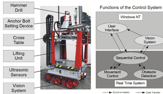
Mobile Construction Robot for the Interior Work – br2 TUM
